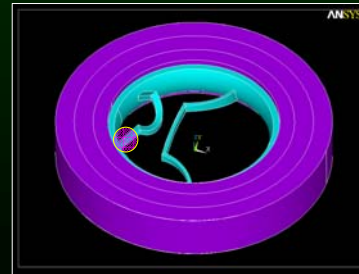
Fig. 10 SLS Valve Model
