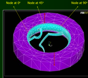
Fig. 8 Harmonic Analysis
